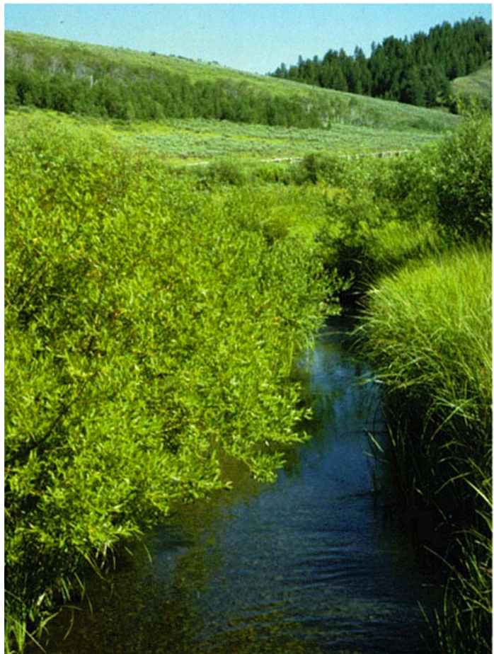
Figure 23 —Example of a healthy riparian area: Cross-Section = PNC; Greenline = PNC; Woody Regeneration = Healthy; and Bank Stability = Excellent.
